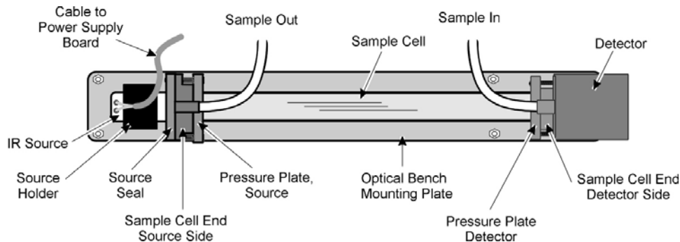
Figure 2-1: Optical Bench Components
