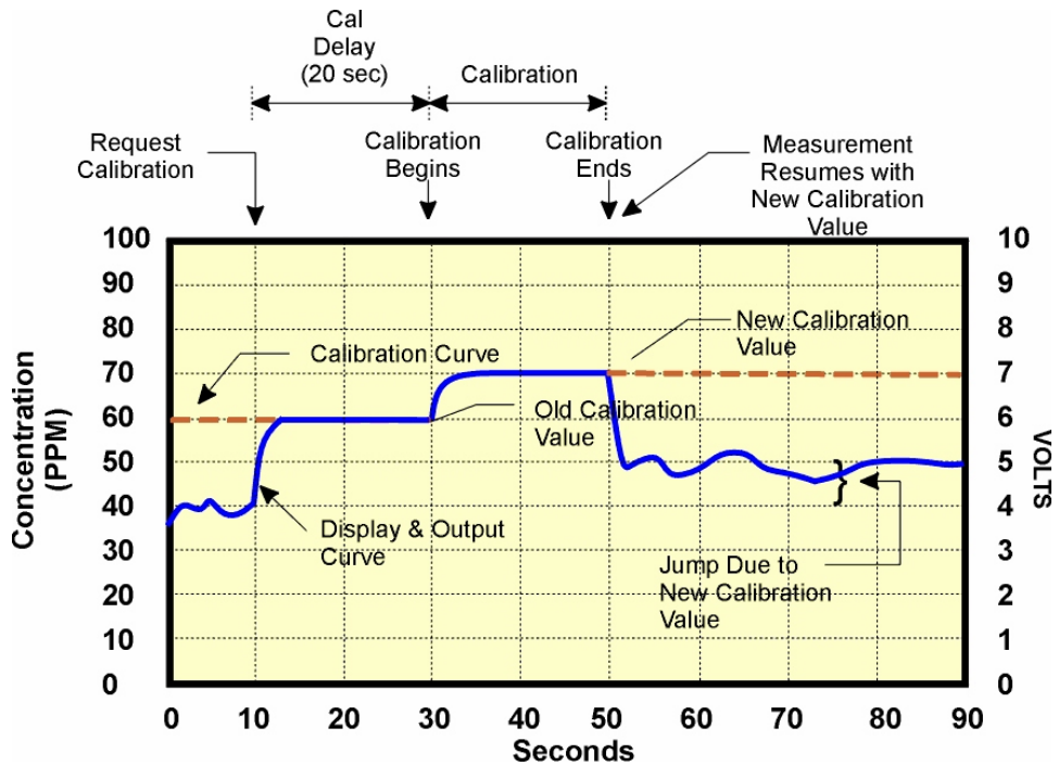
Figure 4-4: Display & Output Jump After New Calibration, CAL=TRACK
