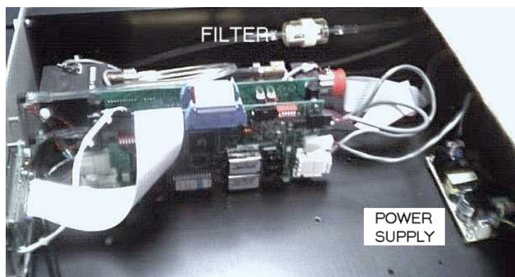
Figure 6-1: Particle Filter Location
