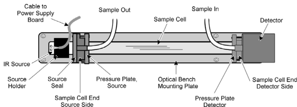
Figure 6-2: Optical Bench Components
