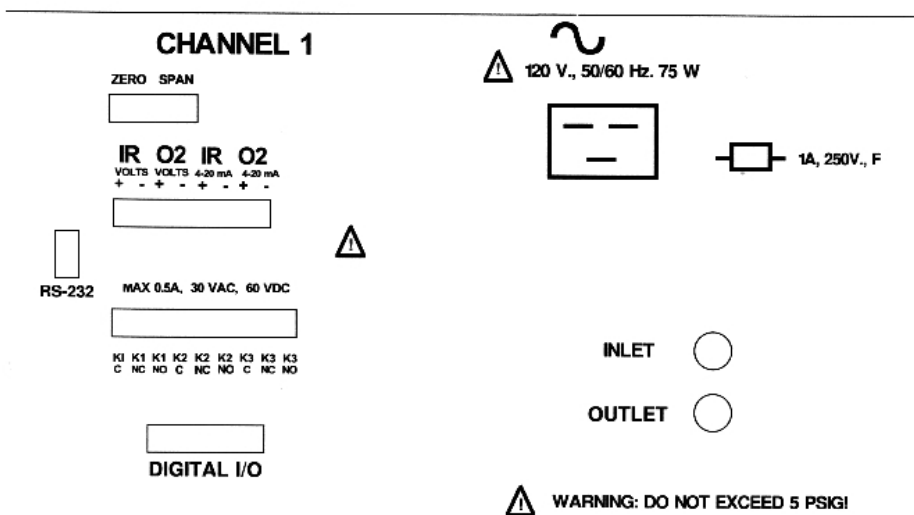
Figure 3-5: IR7000 Rear Panel
