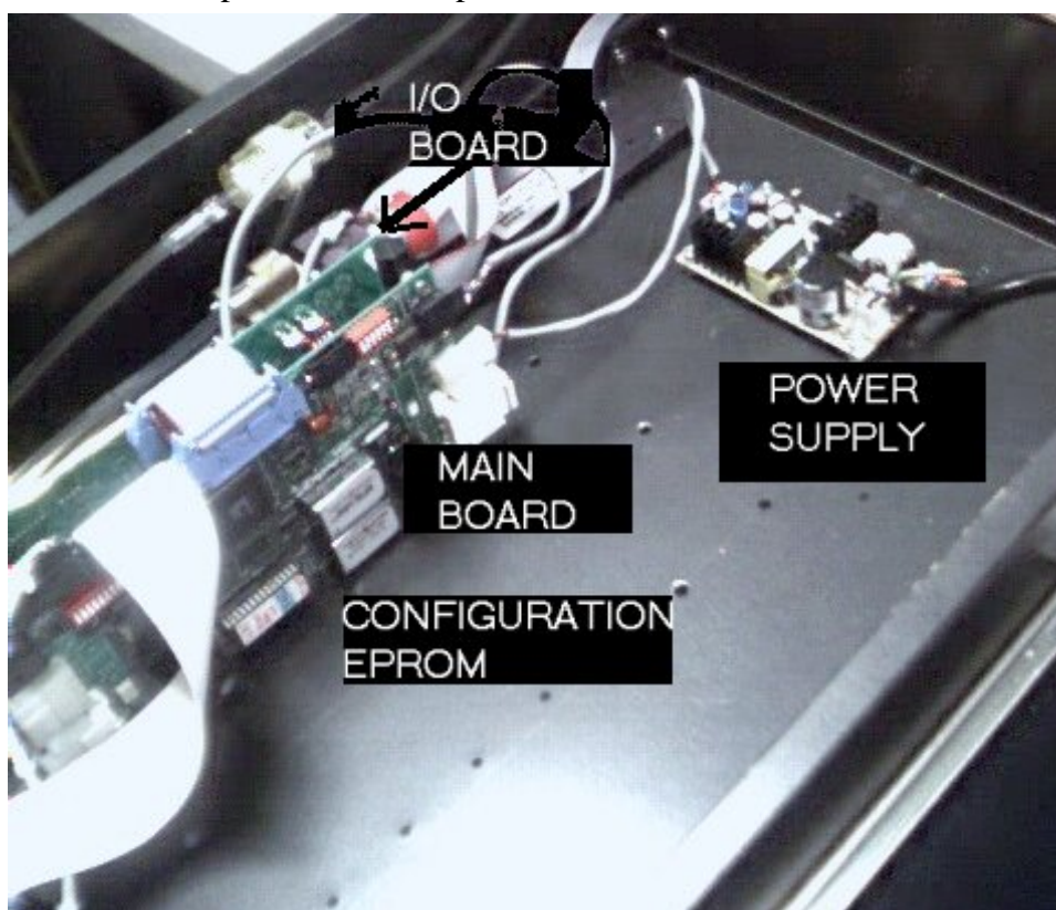
Figure 2-2: PC Board Identification and Location
