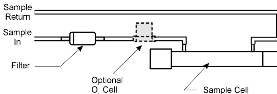
Figure 2-4: Sample Path Through Analyzer – Standard Model
