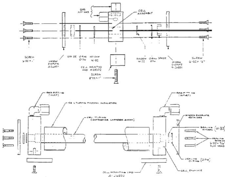
Figure 5-3: Cell Assembly
