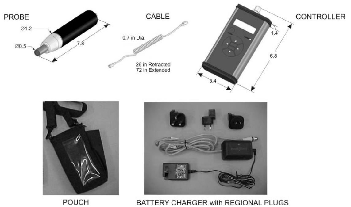
Figure 2-1: Analyzer Components
