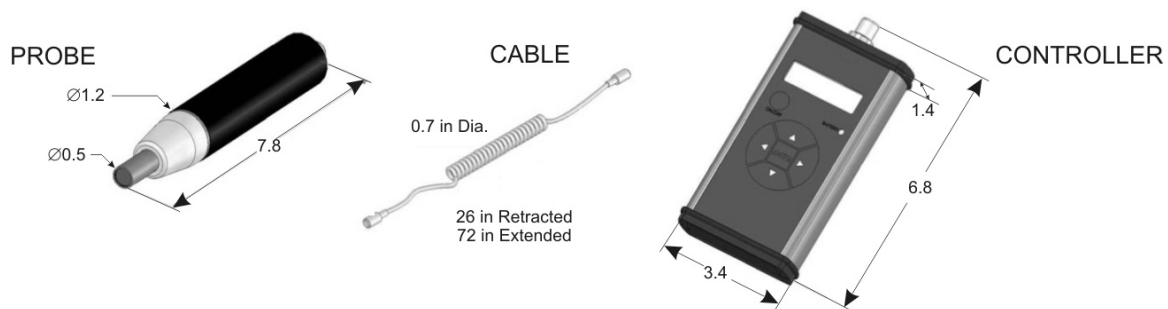
Figure A-1: Dimensions
